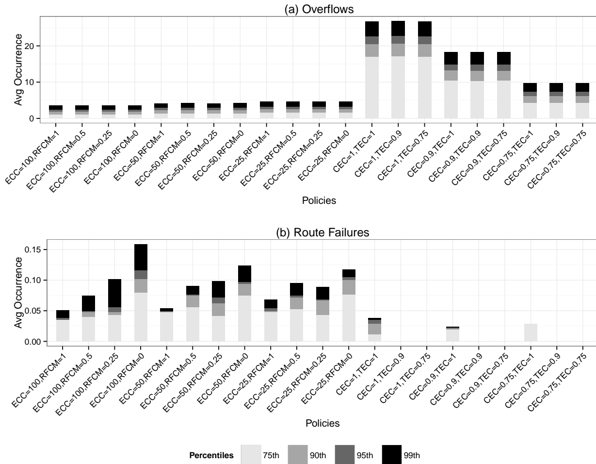
Figure 7 Comparison of Container Overflows and Route Failures for Probabilistic and Alternative Policies
